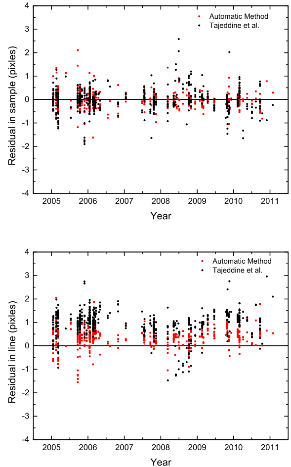
Figure 2. Residuals for all 551 observed positions of Enceladus relative to SAT375 ephemeris in sample and line, respectively. The red dots represent the residuals from the automatic method and the black dots are from Tajeddine et al. (2013). The sample and line is the image coordinate system, and its origin is at the top left of the image with the line, y , increasing downwards and sample, x , to the right.
