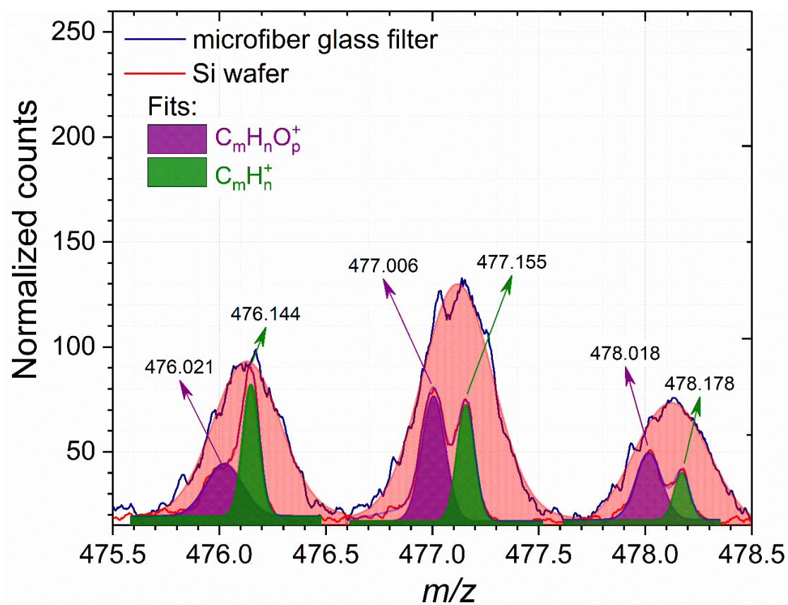
Figure 2. Comparison of mass spectra at m/z = 476 -478 obtained from deposits on glass microfiber filter (dark blue line) and Si wafer (red line). The colored areas below the curves are the Gaussian fits of the deconvoluted peaks.
