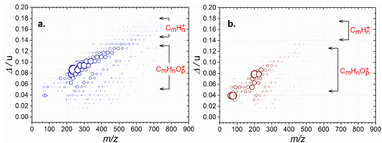
Figure 5. Mass defect plots of soot samples obtained from (a) the soot deposit ROI and (b) the condensable gas ROI. The size of the data points is proportional to the area of the peak normalized to the total ion counts calculated on the selected peak list.
