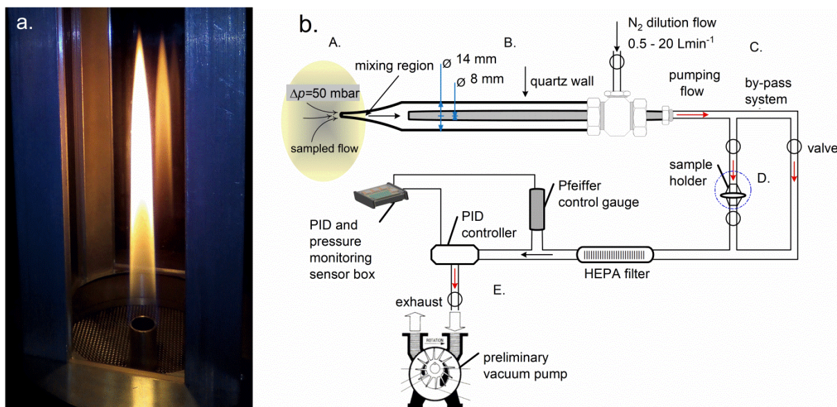
Figure 1. (a) Investigated flame (DIF-S) surrounded by a shielding quartz windowed chimney. During the soot sampling procedure one of the windows is removed for the sampling probe insertion. (b) Overview of the experimental setup used for soot and condensable gas sampling (A) from laboratory diffusion flames. The quartz probe (B) consists of two concentric tubes through which the sampling flow is stabilized. The dilution nitrogen enters the top port, flows between the two quartz tubes up to the probe tip, mixes with the sample flow from the flame and it is removed through a bypass system (C) and impactor (D). The pressure in the line is kept constant using a PID controller and a preliminary vacuum pump (E).
