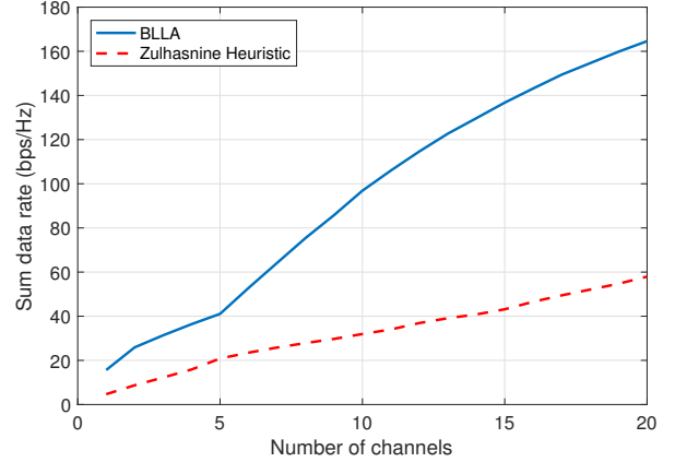
Fig. 8. Normalized sum data rate ( \alpha = 0 ) as a function of the number of channels using BLLA and the heuristic proposed in [13]. The number of UECs are 5 and UEDs are 95. For BLLA, bounded noise is assumed with \ell = 5\% . For [13], full and exact channel information is assumed.
