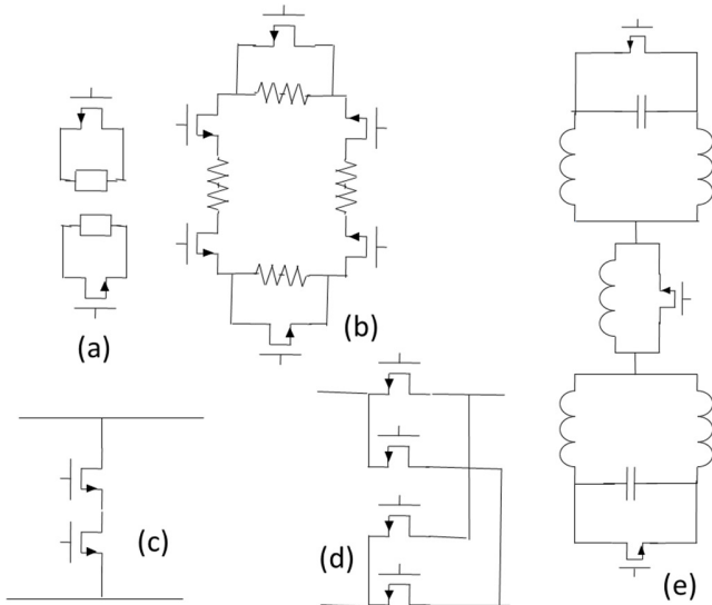
Fig. 1. ideal topologies for Phase Shifters (a)delay line 5,5°, (d)quad-switch 180° and (e)switched filter 11,25°, 22.5°, 45° and 90°) and Attenuators (c)loaded line 0.5dB and 1dB,(b)π-resistive network 2dB, 4dB,and 8dB.
