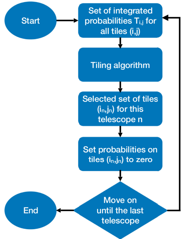
Figure 2. Flowchart of the ‘iterative’ algorithm presented in the text.
