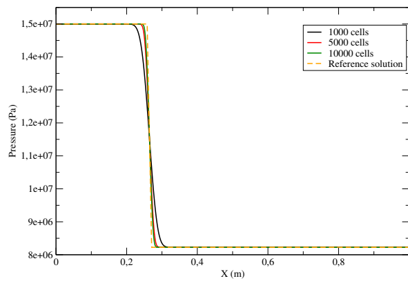
Figure 1.B.6 – Pressure (Pa) as a function of X (m) at the final time compared with the reference solution.
