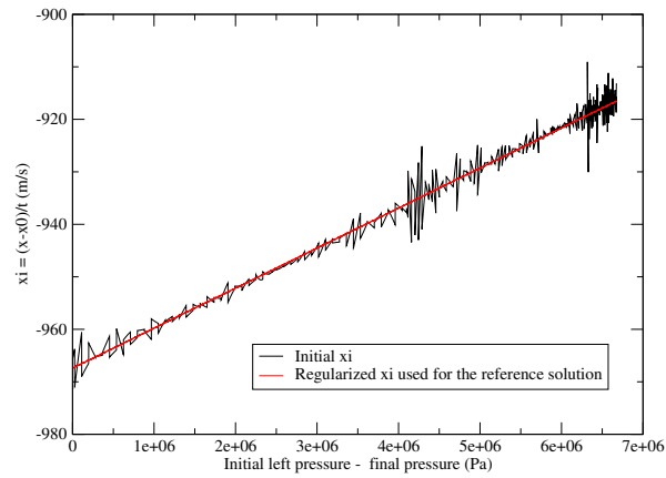
Figure 1.B.4 – \xi^* = \frac{x^* - x_0}{t} = u^* - c^* along the discrete isentropic path and regularized \tilde{\xi} used in the reference solution (abscissas are the opposite of the pressure gap between the final pressure and the initial left pressure equal to 150 \cdot 10^5 \text{ Pa} ).
