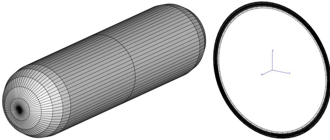
Figure 5. Mesh configuration of the cylinder geometry
