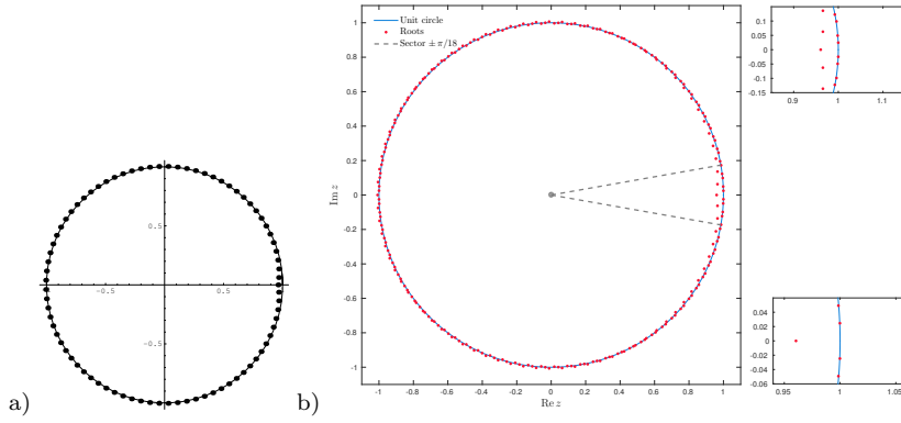
Fig. 4 a) Zeroes of G_{81} , b) Zeroes of f(x) = -1 + x + x^{81} + x^{165} + x^{250} . On the right the distribution of the roots of f is zoomed twice in the angular sector -\pi/18 < \arg(z) < \pi/18 . The number of lenticular roots of f is equal to 5.
