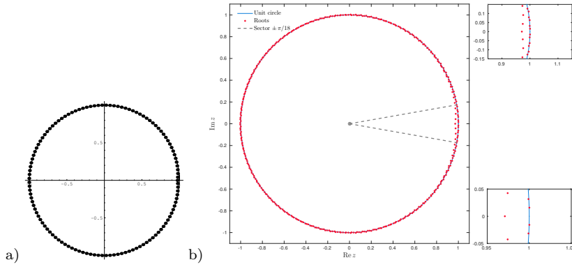
Fig. 5 a) Zeroes of G_{121} , b) Zeroes of f(x) = -1 + x + x^{121} + x^{250} + x^{385} . On the right the distribution of the roots of f is zoomed twice in the angular sector -\pi/18 < \arg(z) < \pi/18 . The lenticulus of roots of f has 7 zeroes.
