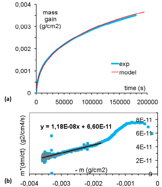
Fig. (6). Thermogravimetry results obtained at 1200°C for the cemented+heat-treated CoTa2, (a) experimental mass gain curve and synthetic curve plotted using the K_p = 66 \times 10^{-12} \text{ g}^2 \text{ cm}^{-4} \text{ s}^{-1} and K_v = 118 \times 10^{-10} \text{ g cm}^{-2} \text{ s}^{-1} values determined in (b) using the m \times \frac{dm}{dt} = K_p - K_v \times m plot.
