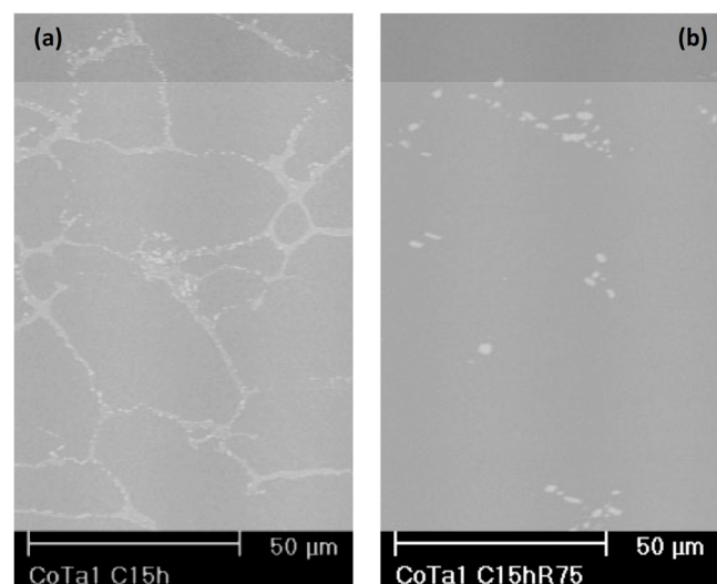
Fig. (11). Comparison of the CoTa1 microstructures after cementation only (a) and after cementation and heat-treatment (b); visualization of the {75h,1200°C} heat-treatment effect on the tantalum-carbides morphology and coarseness.
