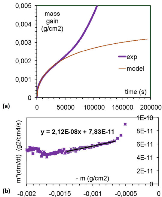
Fig. (5). Thermogravimetry results obtained at 1200°C for the cemented+heat-treated CoTa1, (a) experimental mass gain curve and synthetic curve plotted using the K_p = 78 \times 10^{-12} \text{ g}^2 \text{ cm}^{-4} \text{ s}^{-1} and K_v = 212 \times 10^{-10} \text{ g cm}^{-2} \text{ s}^{-1} values determined in (b) using the m \times \frac{dm}{dt} = K_p - K_v \times m plot.
