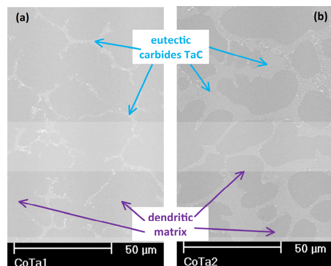
Fig. (1). As-cast microstructures of the studied cobalt-based alloys: (a) CoTa1 and (b) CoTa2 (SEM micrographs in BSE mode).
