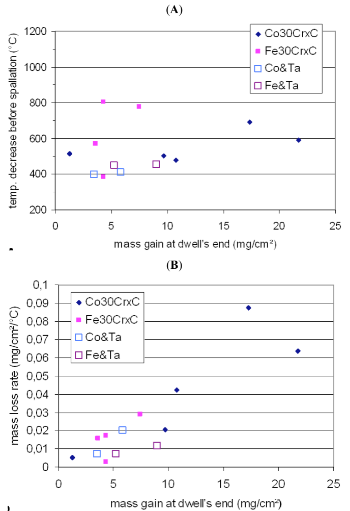
Fig. (11). Difference between the temperature at which spallation begins during cooling and the dwell temperature (A) and rate of mass loss during cooling (B), plotted versus the mass gain isothermally achieved.
