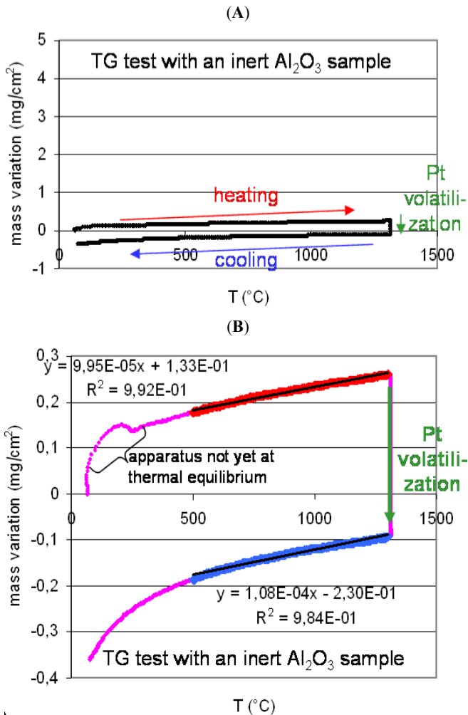
Fig. (2). Mass variations due to the Archimedes' thrust during heating and during cooling: (A) revealed by a test with an \text{Al}_2\text{O}_3 sample with the same geometry as a real alloy sample, and plotted with the same mass gain scale as for to the real alloys when tested until 1000^\circ\text{C} ; (B) enlargement of the previous graph for revealing initial variations due to a thermal equilibrium not yet established at the beginning of the heating part, and measurement of the mass increase rates (divided by 2\text{ cm}^2 , typical average surface of the alloy samples) (same thermobalance as for the alloy samples, heating rate and cooling rate: +20\text{K min}^{-1} and -5\text{K min}^{-1} , dwell at 1300^\circ\text{C} during 10 hours, volatilization of the hottest part of the platinum wires).
