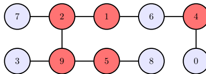
Figure 6: Dominating set (red vertices) identified using our methodology on Figure 3 graph.
