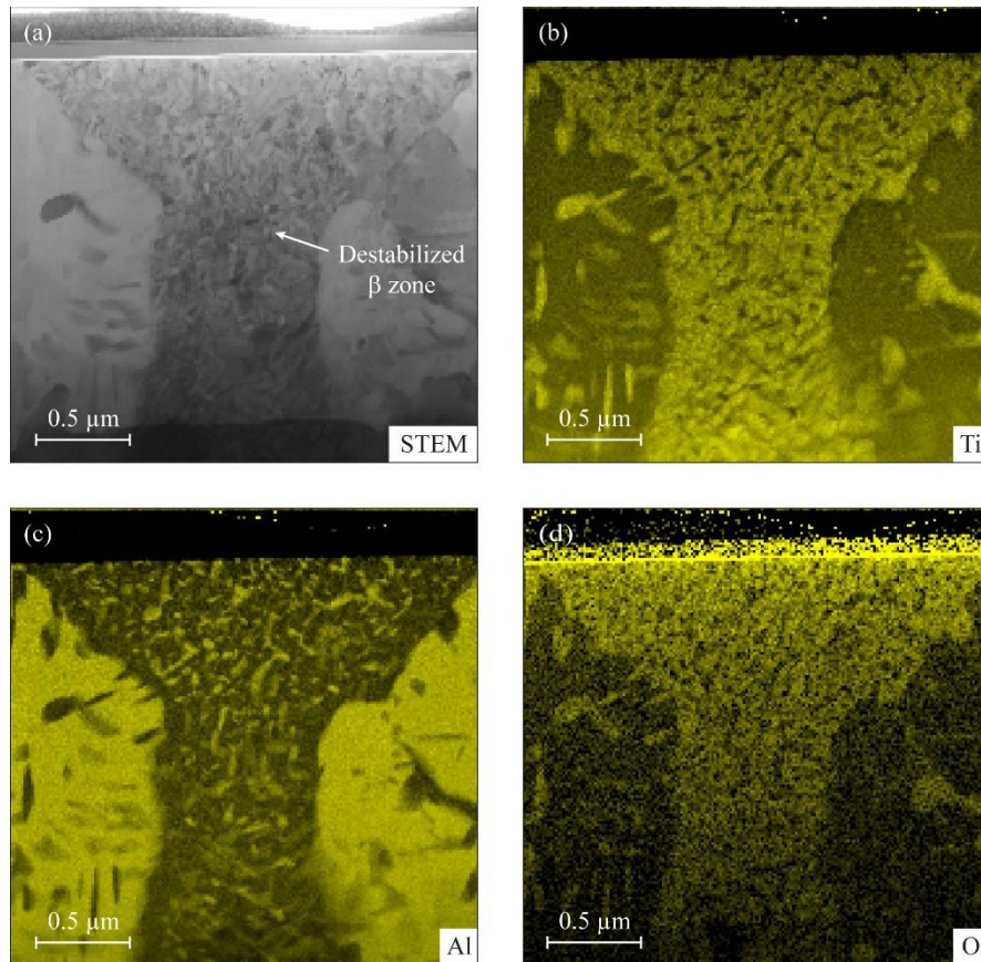
Fig. 8. STEM EDX maps of a destabilized \beta zone (TEM thin foil extracted by FIB). (a) STEM image. (b-d) Maps of Ti, Al and O.
