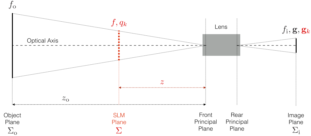
Fig. 1. Conventional approach (black) and proposed approach (red additions). The object f_o that lies on the object plane \Sigma_o is imaged using a conventional optical device with a lens. The numerical image g is formed within the image plane \Sigma_i . Compared to f_i , the ideal geometrical image of f_o , the measured image g suffers from not only sampling, but also diffraction. To circumvent both problems, we place a spatial light modulator (SLM) in the plane \Sigma . From a sequence of modulated images \{g_k\}_{1 \leq k \leq K} acquired using some SLM patterns \{q_k\}_{1 \leq k \leq K} , we can recover f , which is the geometrical projection of f_o onto \Sigma . The dimensions are not to scale, for clarity.
