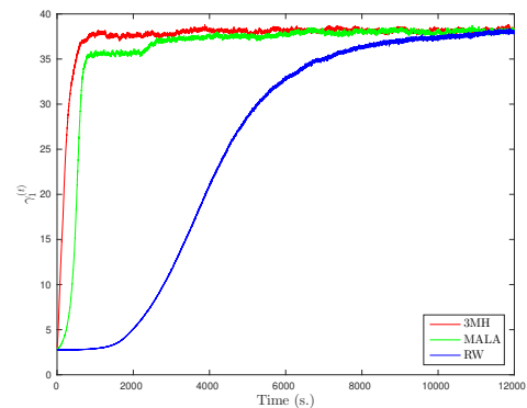
Fig. 1. Convergence speed of RW, MALA and proposed 3MH method.
