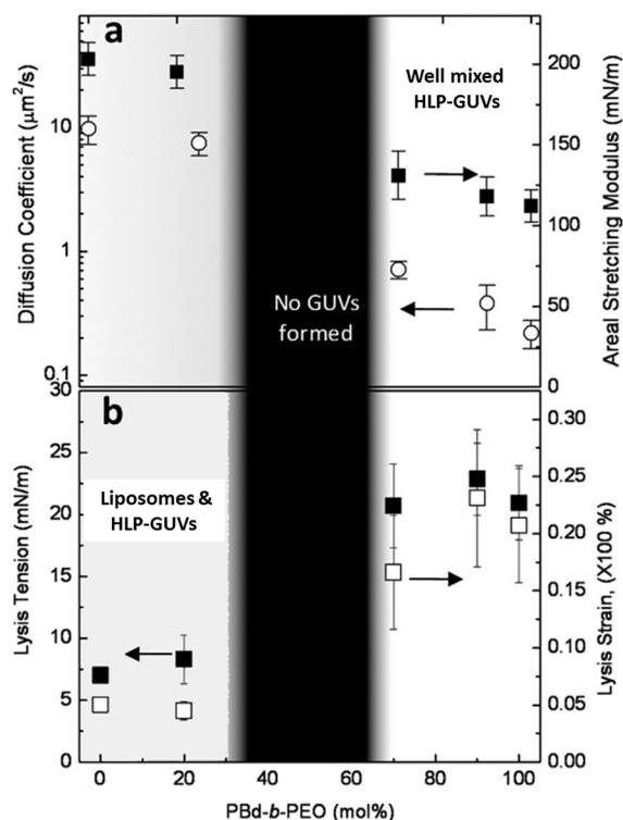
Figure 27-5. (a) Areal stretching modulus K_A (■) and lipid lateral diffusion coefficient D (○) for varying compositions of hGUVs. (b) Critical lysis tension (■) and lysis strain (□) of POPC/PBd- b -PEO GUVs. HLP-GUVs: Hybrid lipid-diblock copolymer giant unilamellar vesicles. Adapted from Nam, J., P. A. Beales, et al. Langmuir 27(1): 1-6. Copyright (2011) American Chemical Society.
