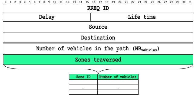
Figure 2: The route request (RREQ) packet format.
