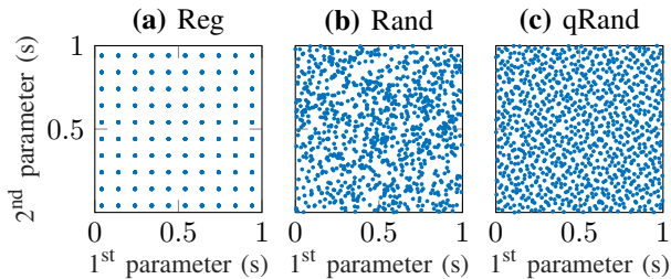
Fig. 1. Illustration of the dictionary sampling strategies. Plots show the 2-dimensional projections of N = 1000 dictionary entries of the 3-dimensional parameter space ( P = 3 ) obtained from (a) a regular grid sampling (Reg), (b) a random sampling (Rand) and (c) a quasi-random sampling (qRand) obtained from a scrambled Sobol sequence.
