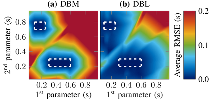
Figure 3: Estimation accuracy outside the limits of the parameter space covered by the dictionary, using synthetic scalable signals: Average RMSE ( M = 2\,000\,000 test signals) in the parameter space ( P = 2 ) obtained (a) with the DBM and (b) with the DBL method. The white dashed lines delimit the subspace covered by the dictionary. The average RMSE is computed from signals in a 50 \times 50 ms sliding window, moving in 5 ms steps in the parameter space.
