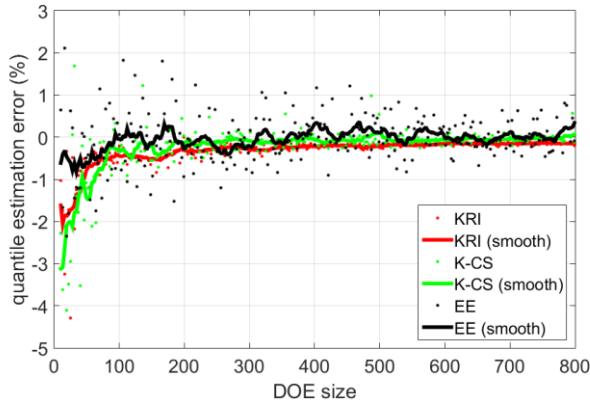
Fig. 7. PCB radiation q_{99\%} estimation: relative error (%) with: Empirical Estimation (EE), kriging (KRI) and kriging + controlled stratification (K-CS).
