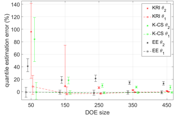
Fig. 2. Reflection coefficient q_{10\%} estimation. Mean relative error ( \theta_1 ) and maximum absolute relative error ( \theta_2 ) with: Empirical Estimation (EE), kriging (KRI) and kriging+controlled stratification (K-CS).
