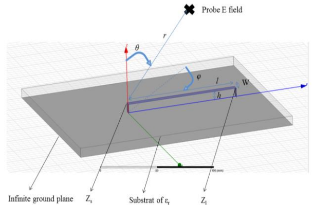
Fig. 4. PCB schematic.
