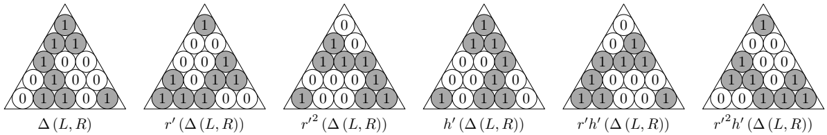
Figure 18: Action of D_3 on \Delta((11100), (11001))
