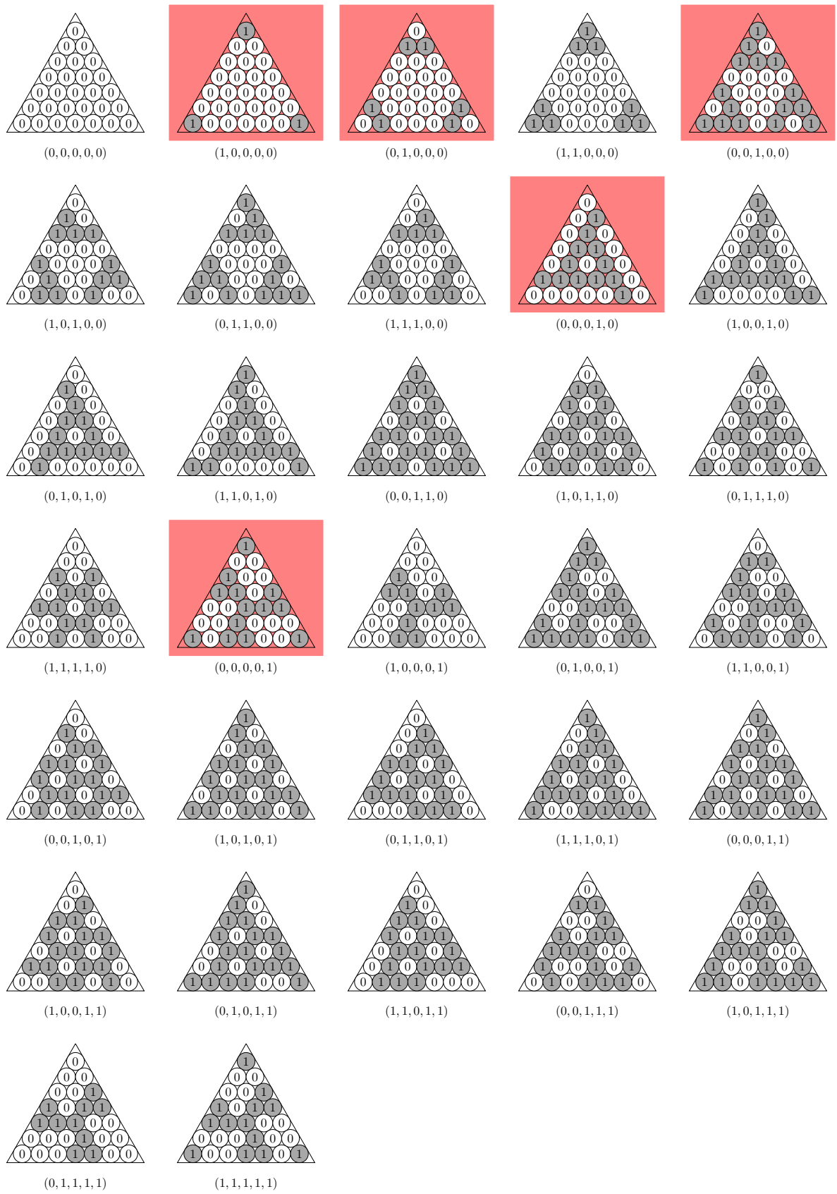
Figure 20: The 32 triangles of \mathcal{RPT}(7) where the 5 red triangles form a basis
