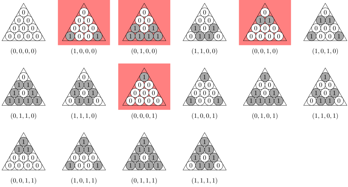
Figure 21: The 16 triangles of \mathcal{HPT}(4) where the 4 red triangles form a basis
