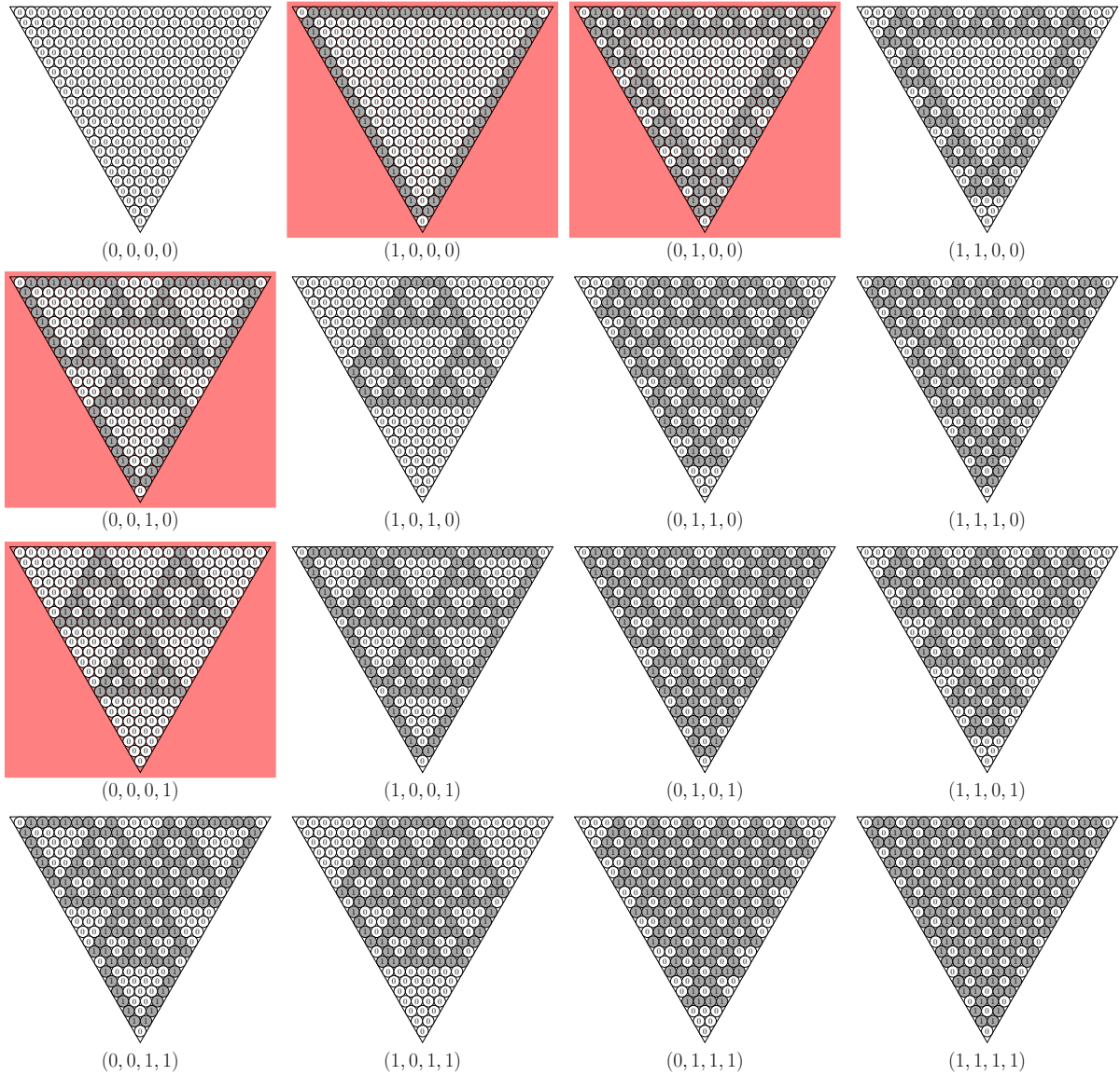
Figure 12: The 16 triangles of \mathcal{DST}(22) where the 4 red triangles form a basis
