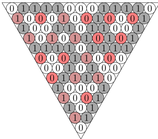
Figure 13: The Steinhaus triangle \theta(G(101000)) where \nabla(101000) appears in red
