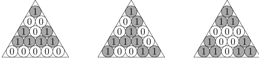
Figure 19: Triangles of \mathcal{HPT}(5) , \mathcal{RPT}(5) and \mathcal{DPT}(5) .
