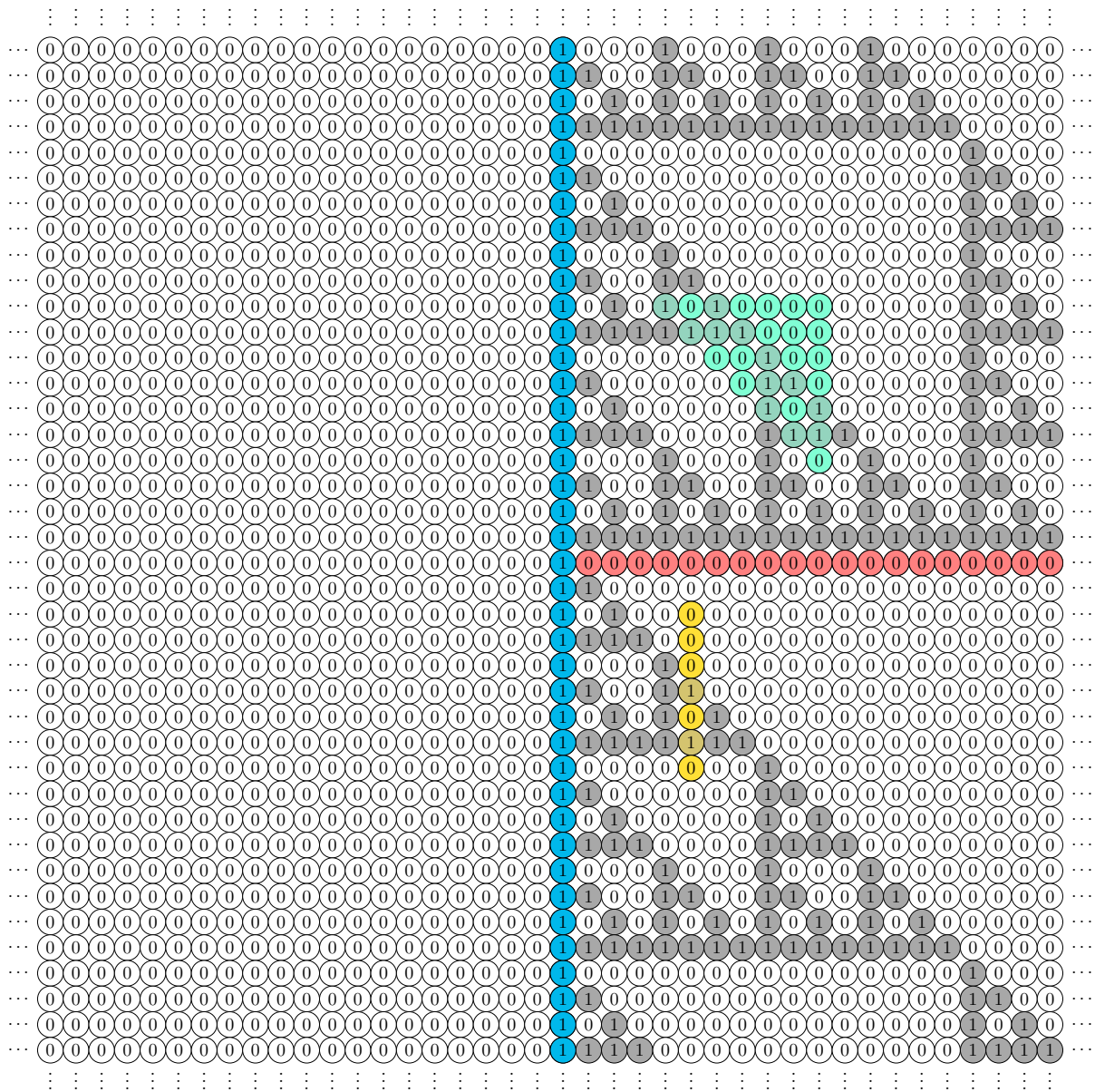
Figure 9: The infinite Pascal matrix modulo 2 with \binom{a}{0}_2 in blue, \binom{0}{b}_2 in red, S_{5,2}^{(7)} in yellow and \nabla S_{10,-10}^{(7)} in green
