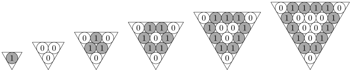
Figure 8: U_n for n \in \{1, \dots, 6\}
