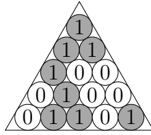
Figure 16: The generalized Pascal triangle \Delta((11100), (11001))
