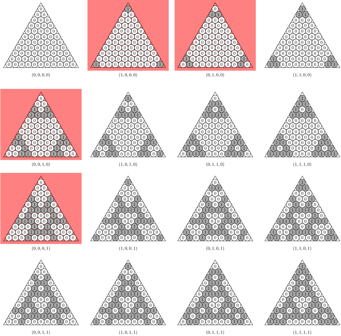
Figure 22: The 16 triangles of \mathcal{DPT}(11) where the 4 red triangles form a basis
