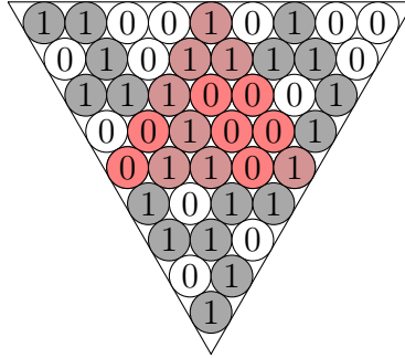
Figure 17: \gamma(\nabla(110010100)) = \Delta((11100), (11001))
