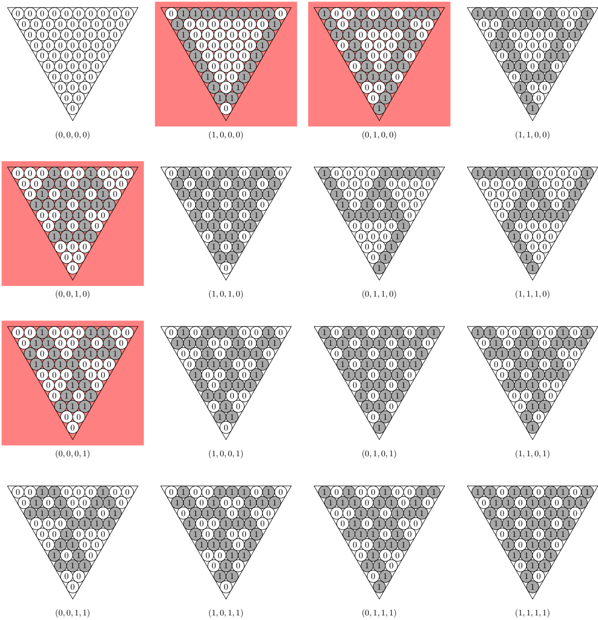
Figure 10: The 16 triangles of \mathcal{RST}(10) where the 4 red triangles form a basis
