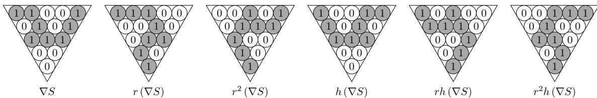
Figure 2: Action of D_3 on \nabla(11001)
