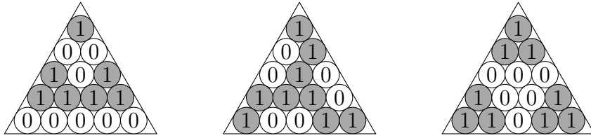
Figure 19: Triangles of \mathcal{HPT}(5) , \mathcal{RPT}(5) and \mathcal{DPT}(5) .
