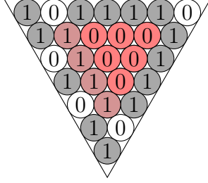
Figure 7: H(\nabla(1011110)) = \nabla(1000)
