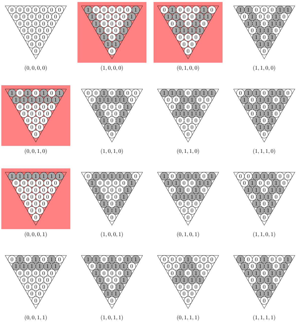
Figure 11: The 16 triangles of \mathcal{HST}(7) where the 4 red triangles form a basis
