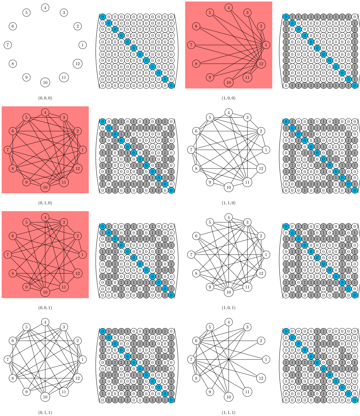
Figure 14: The 8 graphs of \mathcal{E}\mathcal{S}\mathcal{G}(12) where the 3 red graphs form a basis
