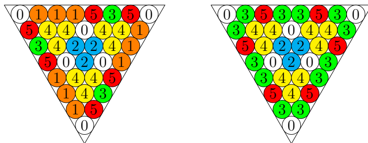
Figure 24: Triangles in \mathcal{RSC}_{(\mathbb{Z}/6\mathbb{Z}, \star)}(8) and \mathcal{DSC}_{(\mathbb{Z}/6\mathbb{Z}, \star)}(8)
