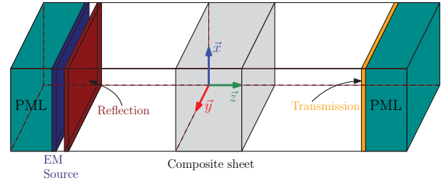
Fig. 3: 3D - Finite element computation domain.
