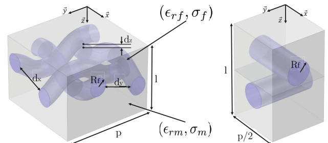
Fig. 9: Woven fiber composite vs. 2 layered unidirectional fiber laminate composite.
