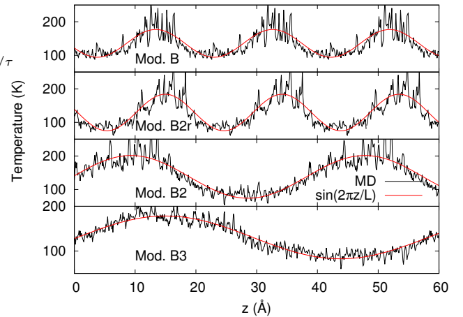
FIG. 6: Temperature profile along the transport direction, averaged during phase 2 of AEMD. The black lines are the MD results. The red lines are sine functions (Eq. 4).
