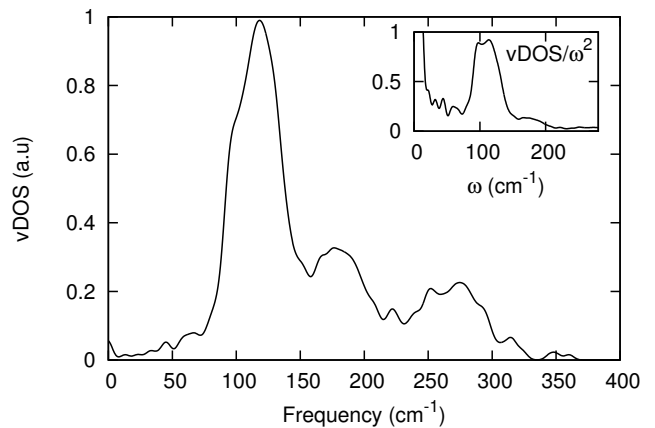
FIG. 2: Vibrational density of states (vDOS). A Gaussian broadening of 5 \text{ cm}^{-1} has been employed. In inset, vDOS divided by the frequency square \omega^2 .
