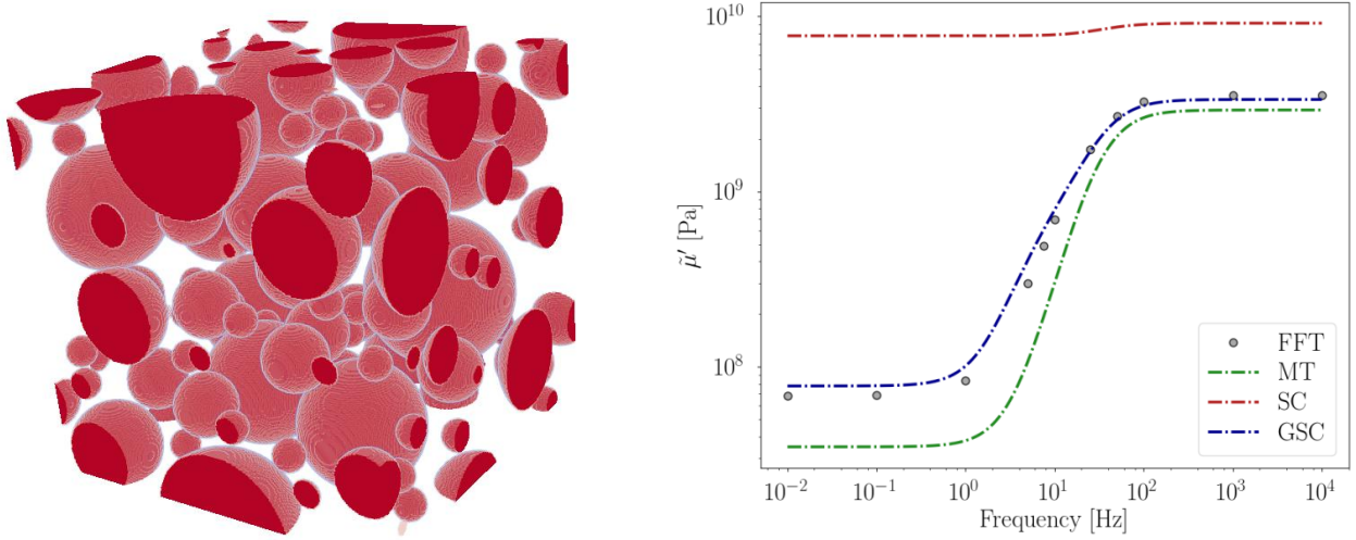
Fig. 12: a (left): the 50% vol. fraction composite of elastic spheres embedded in a Zener matrix used for FFT computations – b (right): comparison between the homogenized shear storage modulus (real part of the complex relaxation function) predicted by the Mori-Tanaka (MT), self-consistent (SC) and generalized self-consistent (GSC) mean-field theories and full-field FFT computations ( Gallican et al., 2018 ).
