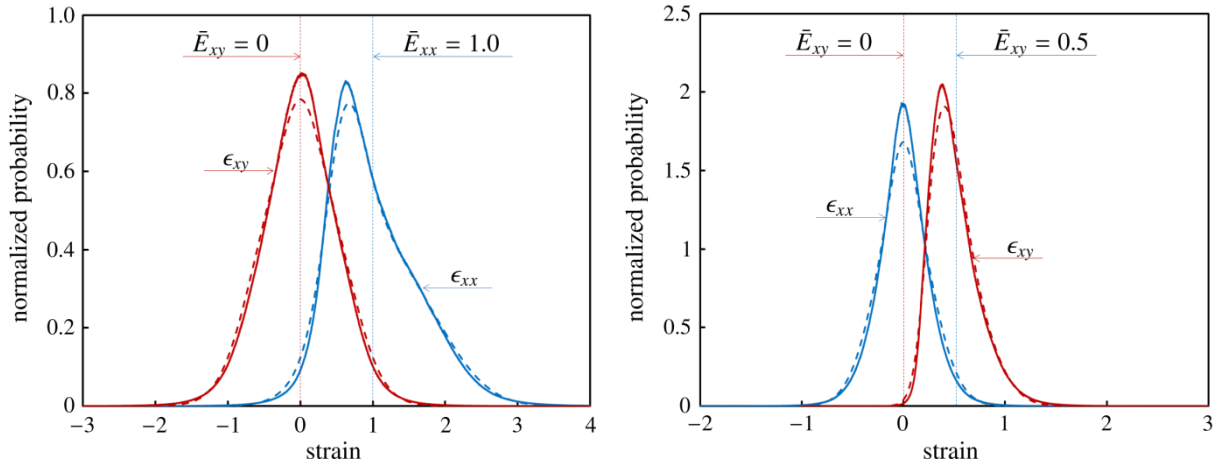
Fig. 11: Distribution functions of some strain fields in the polycrystal continuum: from FFT full-field computations - dashed: reconstructed from self-consistent calculations a (left): hydrostatic loading – b (right): shear loading.
