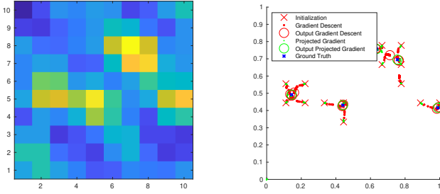
Fig. 2. Result for a few spikes in 2d. Left: back-projection of measurements on a grid. Right: Initialization, gradient descent and projected gradient descent trajectories.
