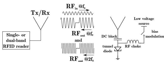
Fig. 1: A concept of the Harmonic Tunneling RFID tag communicating with either a dual-band or a single-band legacy RFID reader.
