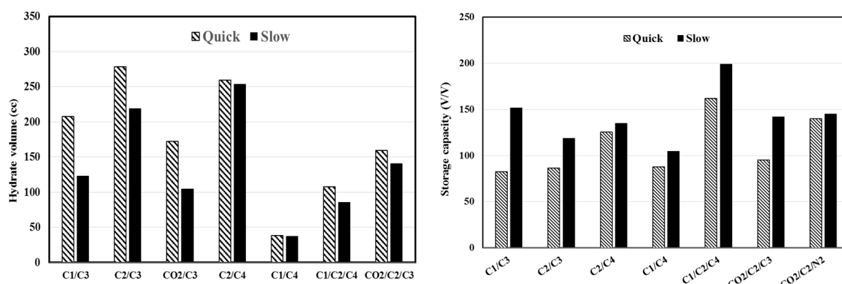
Figure 1: Hydrate volume (left) and storage capacity (right) differences between quick and slow crystallization [3,4]
