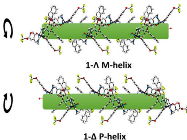
Figure 4. Helical arrangement of the 1- \Lambda (top) and 1- \Delta (bottom) complex viewed along the b-axis which includes the Mn(III) complex cation and (R,R)/(S,S)- \text{X}^- anion around a rod showing the anti-clockwise (M-helix, top) and clockwise (P-helix, bottom) arrangement of cation and anion.
