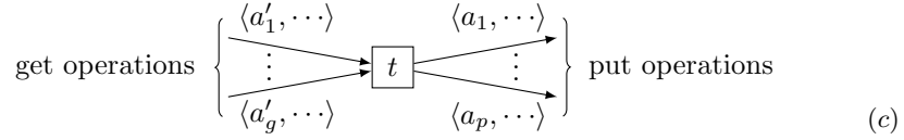
Fig. 1. Parts of the guard and the shape of arcs for assumption 3. In (a) the arcs are connected to the generator place, in (b) to control-flow places, and in (c) to data places. The a_i 's and a'_j 's are variables.
