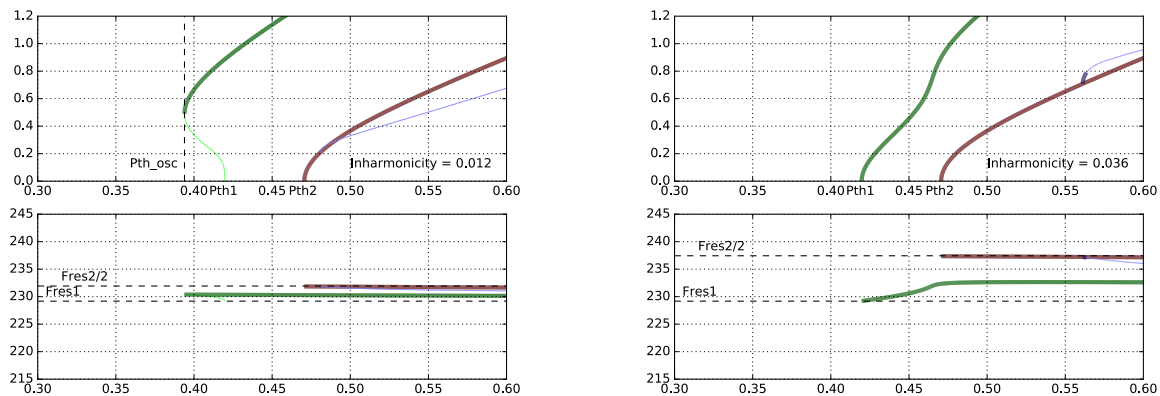
Figure 2: Bifurcation diagrams corresponding to the case of an input instrument with a 1^{st} peak 50% larger than the 2^{nd} one, like in figure 1. The ratio between the two resonance frequencies is 2.024, inharmonicity 0.012 (left) or 2.072, inharmonicity 0.036 (right). Top plots represent the amplitude of the periodic oscillation branches with respect to the blowing pressure. Bottom plots represent the frequency of the corresponding periodic solutions with respect to the blowing pressure. Green (red) lines correspond to periodic oscillations resulting from the instability of the first (second) acoustic resonance and are called 1^{st} and 2^{nd} registers respectively. Blue lines correspond to periodic oscillations of the 1^{st} register resulting from the period doubling of the 2^{nd} register.
