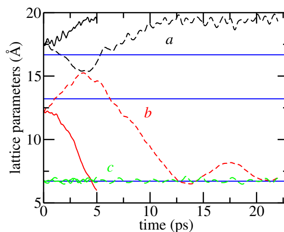
Figure 3. Evolution of the cell parameters at 1 bar, 600 K, with the Grimme dispersion correction (solid line: D2 45 , dashed line: D3 52 ). The experimental lattice parameters 33 for the large-pore phase are shown as blue lines.
