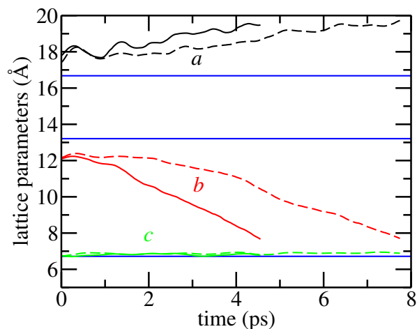
Figure 8. Evolution of the cell parameters at 1 bar, 600 K, with the Dion exchange-correlation functional. Full and dashed lines represent simulations using a single unit cell and a 1 \times 1 \times 2 supercell, respectively. The experimental lattice parameters 33 for the large-pore phase are shown as blue lines.
