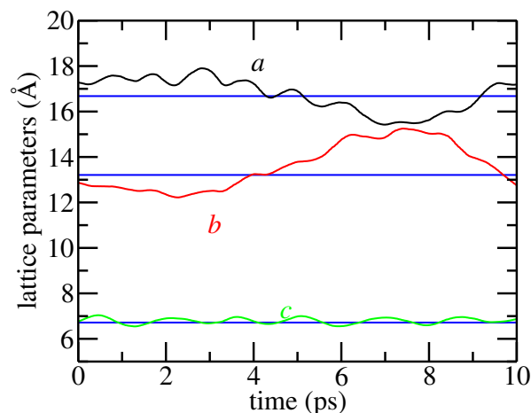
Figure 5. Evolution of the cell parameters at 1 bar, 600 K, with the modified Grimme dispersion correction (global scaling factor s_6 = 0.2 ). The experimental lattice parameters 33 for the large-pore phase are shown as blue lines.
