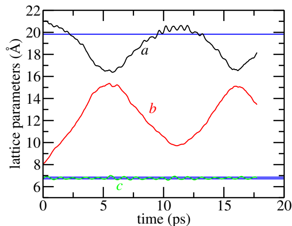
Figure 6. Evolution of the cell parameters at 1 bar, 300 K, with the modified Grimme dispersion correction (global scaling factor s_6 = 0.2 ). The experimental lattice parameters 33 for the narrow-pore phase are shown as blue lines.
