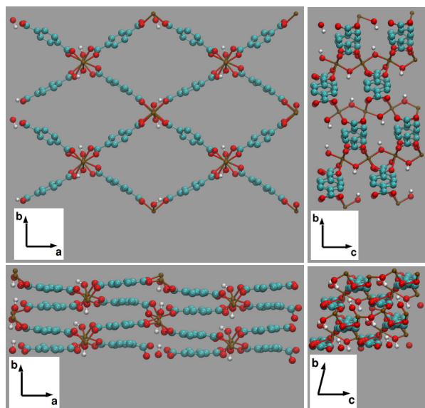
Figure 4. Snapshots from the beginning (upper panel) and the end (lower panel) of the NPT simulation ( P = 1 bar, T = 600 K) with the original Grimme D2 dispersion correction and PBE. The simulation box consists of one unit cell and is repeated periodically here by 2 \times 2 \times 2 units for a better visualization of the structure. For clarity, hydrogen atoms bonded to the benzenedicarboxylate linkers are not shown.
