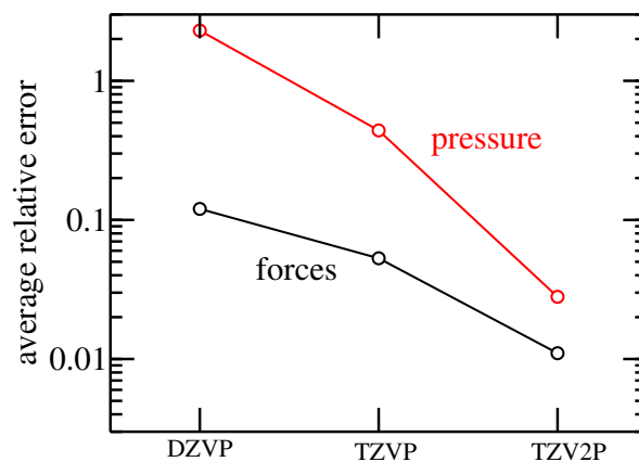
Figure 2. Relative average error of forces and pressure as a function of basis set size, using a very large cutoff ( E_{\text{cut}} = 2500 Ry, E_{\text{cut}}^{\text{rel}} = 100 Ry).
