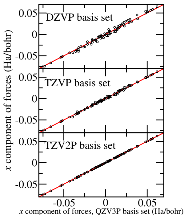
Figure 1. Convergence of forces with basis set size, using a very large cutoff ( E_{\text{cut}} = 2500 Ry, E_{\text{cut}}^{\text{rel}} = 100 Ry).
