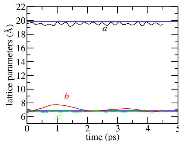
Figure 7. Evolution of the cell parameters of the narrow-pore phase, at 1 bar and 300 K, with the Dion exchange-correlation functional. The experimental lattice parameters 33 for the narrow-pore phase are shown as blue lines.
