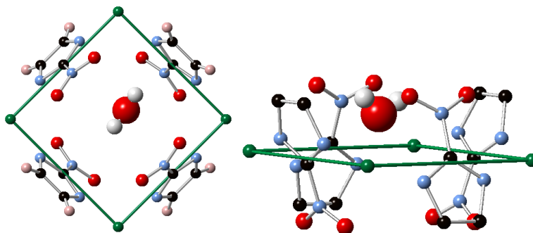
Figure 8. Snapshot of the 4-ring water adsorption site of the ZIF-65 (SOD) material in the gas phase.
