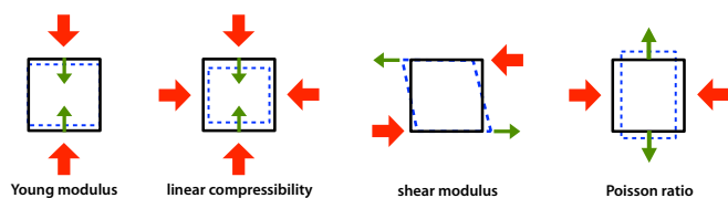
Figure 2. Scheme of the directional elastic properties calculated in this work. For each, large red arrows represent the direction of applied stress and smaller green arrows the direction along which the resulting strain is measured.
