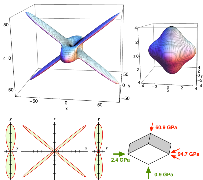
Figure 3. Directional Young modulus for MIL-53(Al)-lp and ZIF-8 represented as 3D surfaces, with axes tick labels in GPa (top left and right, respectively); projection in the xy , xz and zy planes (bottom left; one tick is 10 GPa). A scheme showing the stiffest and weakest directions of the lozenge-shaped pore is presented at the bottom right.
