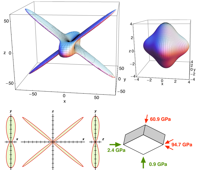
Figure 3. Directional Young modulus for MIL-53(Al)-lp and ZIF-8 represented as 3D surfaces, with axes tick labels in GPa (top left and right, respectively); projection in the xy , xz and zy planes (bottom left; one tick is 10 GPa). A scheme showing the stiffest and weakest directions of the lozenge-shaped pore is presented at the bottom right.
