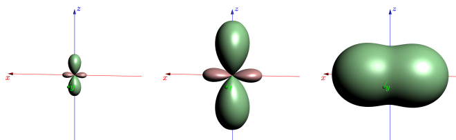
Figure 5. 3D surface representation of the Linear Compressibility of MIL-53(Al)-lp, DMOF1-loz and DMOF1-sq. Positive LC is indicated as green, negative LC in red. The leftmost two are at the same scale (axis length is 1500 \text{ TPa}^{-1} ) while the last one is enlarged 50 times for clarity (axis length is 30 \text{ TPa}^{-1} ).
