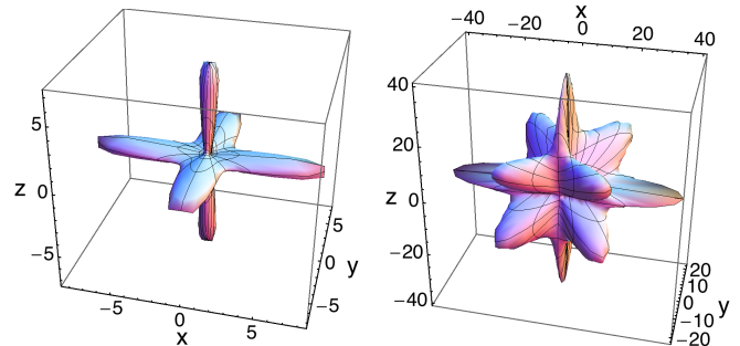
Figure 4. 3D representations of the shear modulus for MIL-53(Al)-lp. Left: minimal shear modulus G_{\min}(\theta, \phi) = \min_{\chi} G(\theta, \phi, \chi) ; right: maximal shear modulus G_{\max}(\theta, \phi) = \max_{\chi} G(\theta, \phi, \chi) . Axes tick labels are in GPa.
