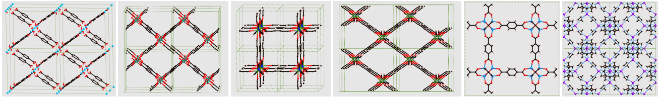
Figure 1. From left to right: MIL-53(Al) lp structure, MIL-47, DMOF1-sq, DMOF1-loz, MOF-5, and ZIF-8.
