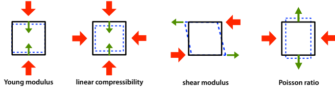
Figure 2. Scheme of the directional elastic properties calculated in this work. For each, large red arrows represent the direction of applied stress and smaller green arrows the direction along which the resulting strain is measured.
