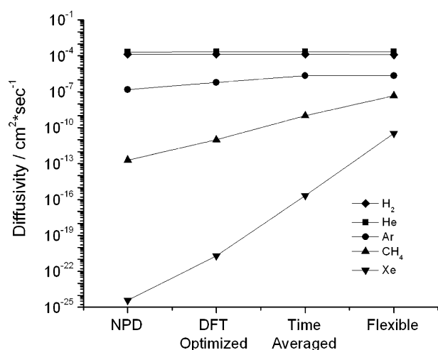
Fig. 1 Diffusivities in the infinite dilution limit for five gases (hydrogen, helium, argon, methane and xenon) with four different computational models of the ZIF-8 framework at 300 K. Figure taken from Ref. 15.
