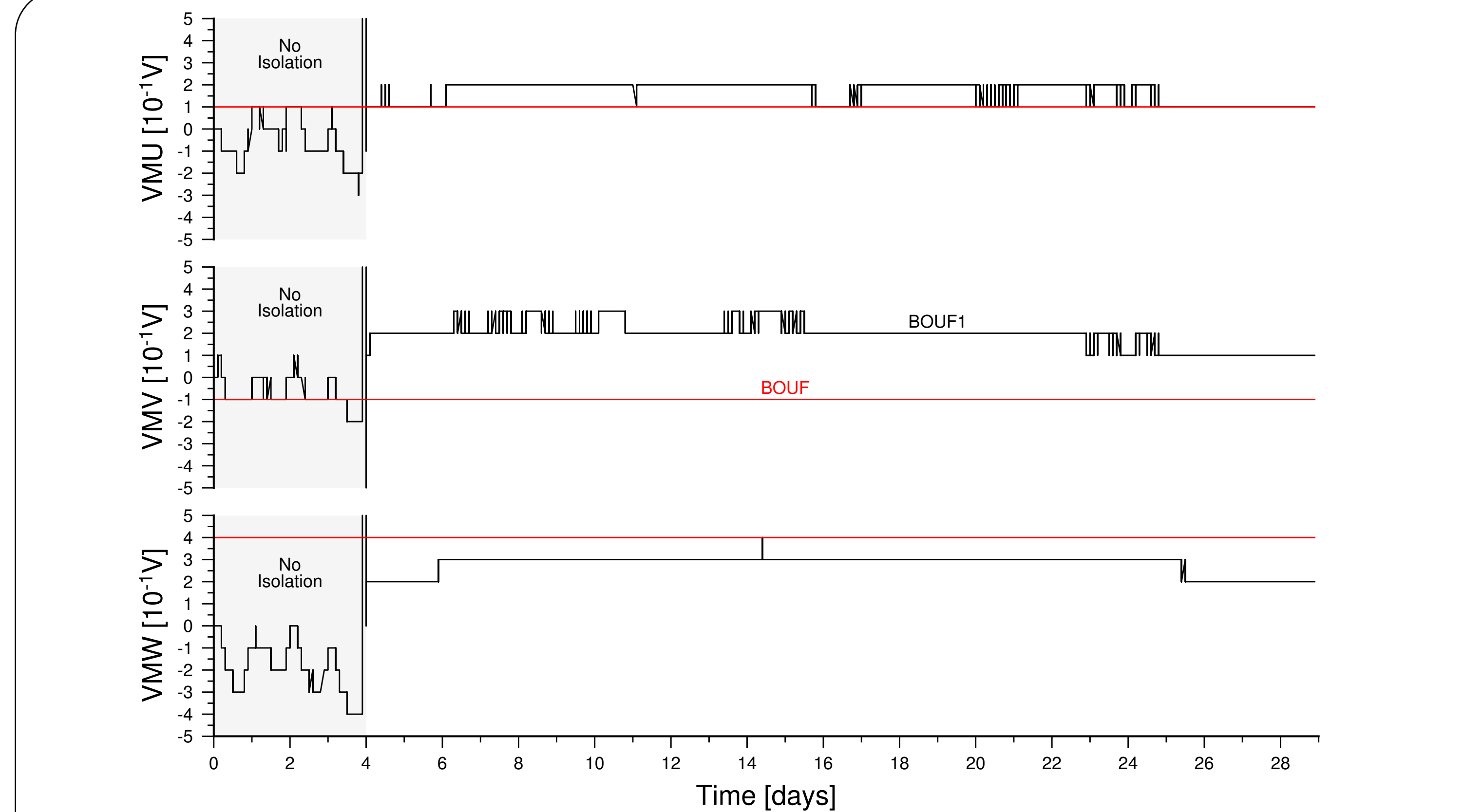
Figure 7: Comparison of the mass position of the T120PA (black) and T120PH (red) sensors on 29 days. Note that T120PA was not isolated for the first 4 days (gray shaded time period).
