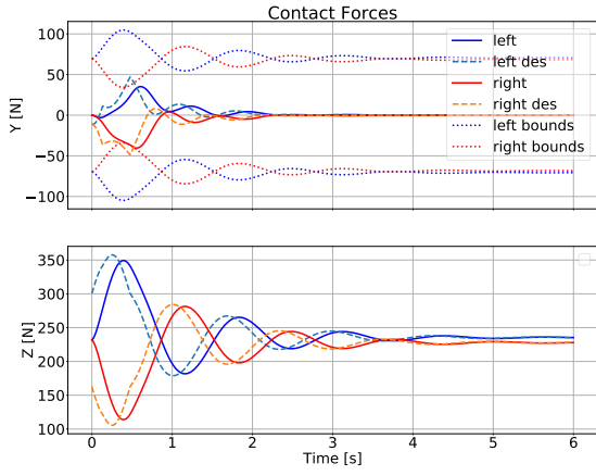
(a) Contact force tracking.
