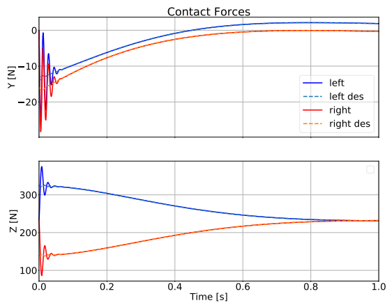
Fig. 6: Contact force generated by TSID-Rigid with stiff contacts, noiseless simulation.
