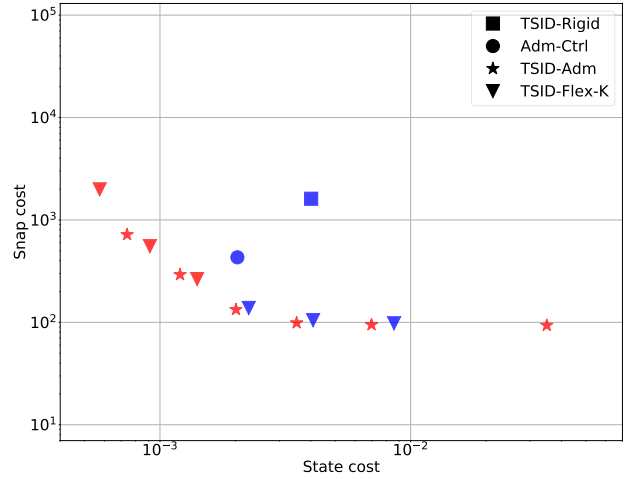
Fig. 4: Results for soft contacts ( \alpha = 0.01 ) and noisy simulation, but without Coulomb friction. Coulomb friction has a detrimental effect to the performance of TSID-Flex-K and TSID-Adm, while it helps stabilizing TSID-Rigid.
