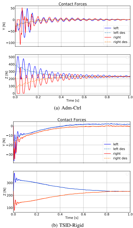
Fig. 8: Stiff contacts, noisy simulation.
