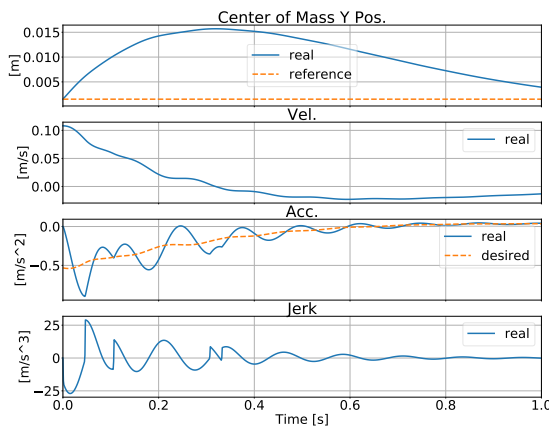
Fig. 3: Performance of TSID-Rigid with soft contacts in noiseless simulation.
