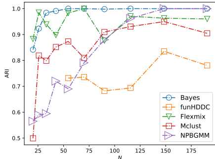
(a) Gaussian perturbations
