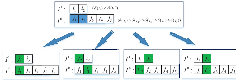
Fig. 2. An illustrative example for the neighborhood generation strategy, where the size of set N and the value of m are respectively 7 and 2, and the size of subset X is 2.
