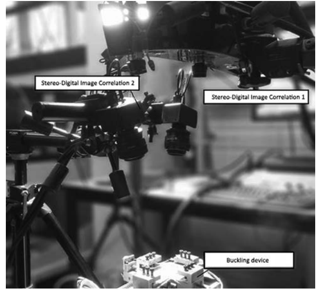
Fig. 2. S-DIC setups with the buckling device.
