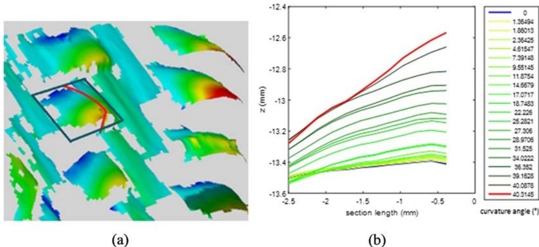
Fig. 4. (a) Reconstructed reinforcement surface by S-DIC (color corresponding to increasing height from blue to red), (b) Profile of a buckle for different bending angles. (For interpretation of the references to color in this figure legend, the reader is referred to the web version of this article.)
