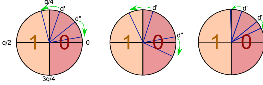
Fig. 4. Left: given that d', d'' \in [0, \frac{q}{4}) , there is no simple way to determine if d' + d'' \in (\frac{q}{4}, \frac{3q}{4}) , i.e. this is a hard case. Adding some \delta to d' while subtracting the same \delta from d'' yields a new pair (d', d'') which is an easy case. Middle: for some hard cases, adding and subtracting a constant \delta does not give a solution: the new pair (d', d'') is another hard case. Right: d' is closer to \frac{q}{4} than d'' is to 0. We therefore let \delta = 1 + \lfloor \frac{q}{4} \rfloor - d' . Then by construction, d' + \delta changes quadrant while d'' - \delta does not. It follows that d = d' + \delta + d'' - \delta > \frac{q}{4} and d < \frac{3q}{4} . Therefore (d', d'') decodes to 1.
