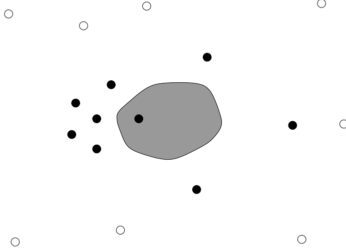
Figure 1: Here E = \mathbb{R}^2 , D is a discrete set of irregularly spaced points, and we take the Euclidean distance d_2 . A compact set K (in grey), and its greatest Hausdorff discretization (shown with filled dots), which consists of all points of D whose distance to K is at most r_H(K) .
