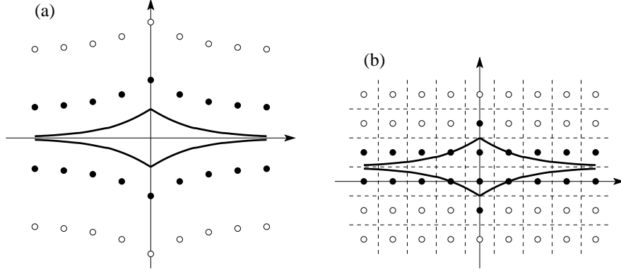
Figure 5: Let E = \mathbb{R}^2 with d induced by the L_\infty norm. In both cases (a,b), the elements of \Delta_H(F) are shown as filled disks, and those of D \setminus \Delta_H(F) as hollow disks. (a) Here D = \{(z, \pm(2n+1+2^{-|z|})) \mid z \in \mathbb{Z}, n \in \mathbb{N}\} , F = \{(y, \pm 2^{-|y|}) \mid y \in \mathbb{R}\} , and r_H(F) = 1 . For all s > 0 , G_{r_H(F)+s}(\Delta_H(F)) is connected, but G_{r_H(F)}(\Delta_H(F)) is not connected. (b) Here D = \mathbb{Z}^2 , F = \{(y, \frac{1}{2} \pm 2^{-|y|}) \mid y \in \mathbb{R}\} , and r_H(F) = r_c = 1/2 . Then G_{r_H(F)}(\Delta_H(F)) is connected, but G_{r_H(F)}^F(\Delta_H(F)) is not connected, and \Delta_H(F) is not chained by the \Delta_{r_H(F)}(x) \cap \Delta_H(F) for x \in F .
