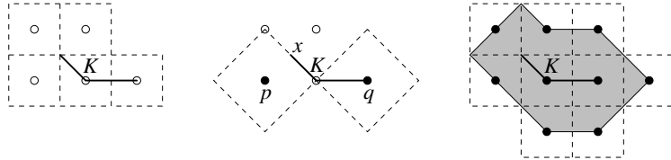
Figure 8: Here E = \mathbb{R}^2 , D = \mathbb{Z}^2 and d is the metric induced by the L_1 norm. Left: the connected compact K \subseteq E and the 5 pixels in D whose square cells intersect K . Middle: the endpoint x of K satisfies d(x, D) = 1 = r_c , hence r_H(K) = 1 ; now H_d(K, \{p, q\}) = 1 , so \{p, q\} is a 8-disconnected Hausdorff discretization of K . Right: the greatest Hausdorff discretization \Delta_H(K) = \delta_1(K) \cap D is 4-connected.
