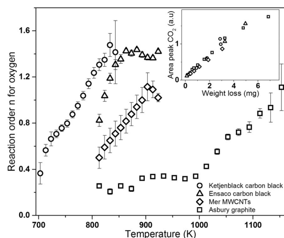
Figure 3. Evolution of the reaction order for oxygen with temperature from the shrinking core model during thermal oxidation. Insert: Correlation between TGA and GC-MS. Residual \text{CO}_2 at 0 mg weight loss comes from air.
