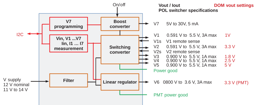
Fig. 13 Block diagram of the power board functionality. The specification of the dc/dc converters is presented for each power rail. The linear regulator included in the power board is used to provide a stable voltage to the PMTs.
