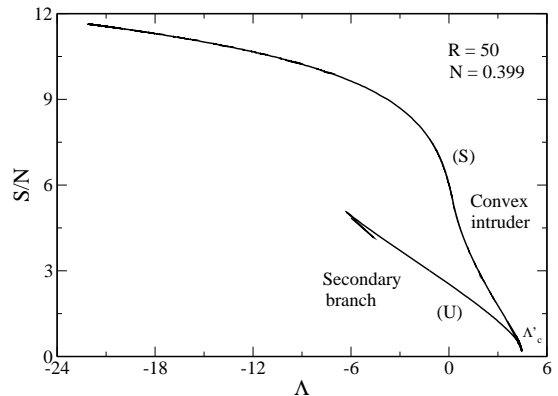
FIG. 3: Entropy per fermion as a function of the normalized energy for N_{\text{OV}} < N \ll N_{\text{max}} (specifically R = 50 and N = 0.399 ). (S): stable; (U): unstable in the MCE.
