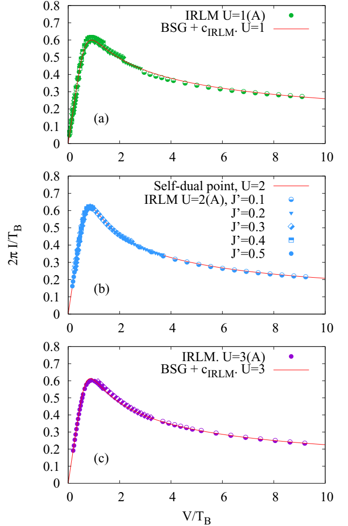
FIG. 6. Rescaled I-V curves for different values of interaction, measured using the protocol (A). U = 1 (a), U = 2 (b), and U = 3 (c). The symbol shapes encode J' . As expected the agreement between the IRLM numerics and the BSG is excellent for U = 2 (self-dual point), but it is also very good for U = 1, 3 where the models are a priori not equivalent.
