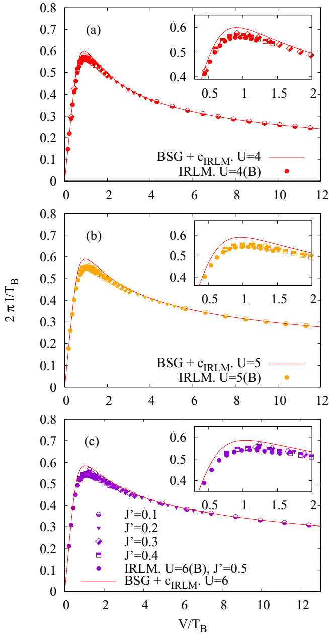
FIG. 7. Same as Fig. 6 for U = 4 (a), U = 5 (b), and U = 6 (c), using the quench protocol (B). The data depart (insets) from the BSG curves [Eqs. (11) and (10)] in the vicinity of V/T_B \simeq 1 .
