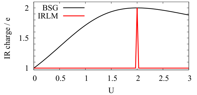
FIG. 12. Charge of quasiparticles dominating transport in the deep IR for the IRLM and BSG model. The charge for the IRLM differs from e only at the self-dual point where it becomes equal to 2e , whereas the charge for the BSG model is a nontrivial function of the interaction parameter U .
