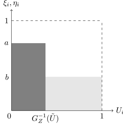
Figure 7: In gray, the domain to which the couple (U_i, \xi_i, \eta_i) needs to belong to from the equation (23). We put \xi_i and \eta_i on the same axis as they do not depend one on the other so that the volume \mathcal{V}(\mathcal{D}) is equal to the sum of the two grey areas.
