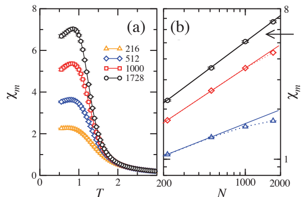
FIG. 8. (Color online) (a) Plots of the magnetic susceptibility \chi_m vs T for \sigma = 0.6 . \Delta , \diamond , \square and \circ stand for systems with N = 216, 512, 1000 and 1728 dipoles respectively. Solid lines are guides to the eye. (b) Log-log plots of \chi_m vs N for \sigma = 0.6 . \circ , \diamond , and \Delta stand for temperatures T = 0.55, 1.25 , and 1.55 respectively. As stressed by the dotted lines connecting the points, data ceases to grow linearly (the solid lines) at large temperatures. The arrow marks the onset of the PM phase.
