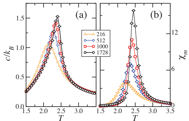
FIG. 4. (Color online) (a) Plots of the specific heat versus T for \sigma = 0.3 . \triangle , \diamond , \square and \circ stand for systems with N = 216, 512, 1000 and 1728 dipoles respectively. (b) Plots of the magnetic susceptibility \chi_m vs T for \sigma = 0.3 . Same symbols as in (a). Lines in both panels are guides to the eye.
