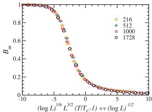
FIG. 6. (Color online) Finite size scaling plots for B_m vs L^{3/2} \log^{1/6} L (T/T_c - 1) + v (\log L)^{-1/2} for \sigma = 0.3 using T_c = 2.57(2) and v = -1.83(8) . \Delta , \diamond , \square and \circ stand for systems with N = 216, 512, 1000 and 1728 respectively.
