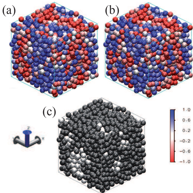
FIG. 1. (Color online) (a) and (b) show two statistically independent configurations of a sample with 1728 magnetic nanospheres with \sigma = 0.6 at the temperature T = 0.55 . The position of the spheres and the orientation of their local easy axes are both frozen. The color of each sphere i stands for the value of the z component of the magnetic moment \tilde{\mu}_i/\mu = s_i \hat{a}_i , where \hat{a}_i is the local easy-axis and s_i = \pm 1 . Picture (c) represents the overlap between the configurations (a) and (b). Black (white) color of spheres in (c) means s_i^{(a)} s_i^{(b)} = +1 ( -1 ).
