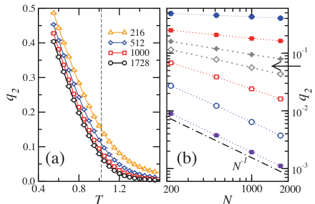
FIG. 11. (Color online) (a) Plots of the squared overlap parameter q_2 vs T for \sigma = 0.6 . \Delta , \diamond , \square and \circ stand for N = 216, 512, 1000 and 1728 respectively. The dashed vertical line indicates the SG transition temperature. Solid lines are guides to the eye. (b) Log-log plots of q_2 vs the number of dipoles N for \sigma = 0.6 . From top to bottom, \bullet , \blacksquare , \blacklozenge , \diamond , \square , \circ , and \Delta stand for T = 0.55, 0.85, 1.0, 1.05, 1.25, 1.55, and 2.55 respectively. The arrow marks the onset of the PM phase. Dotted lines are guides to the eye. The dot-dashed line shows the N^{-1} decay expected for the PM phase.
