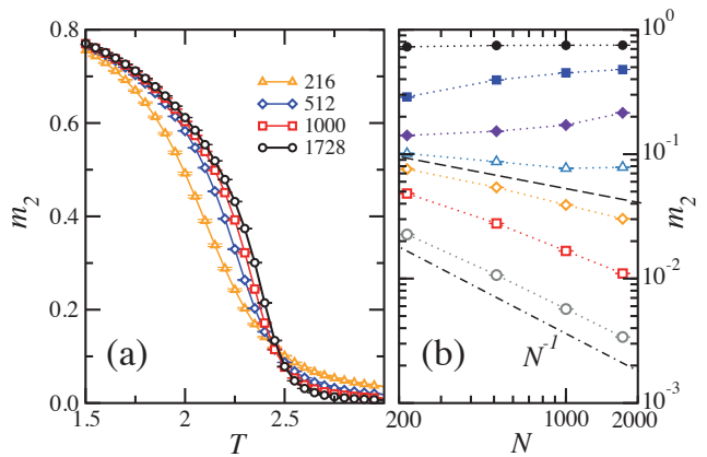
FIG. 3. (Color online) (a) Plots of the squared magnetization m_2 vs temperature T for \sigma = 0.3 . \triangle , \diamond , \square and \circ stand for N = 216, 512, 1000 and 1728 dipoles respectively. Lines are guides to the eye. (b) Log-log plots of m_2 vs N for different temperatures at \sigma = 0.3 . From top to bottom, \bullet , \blacksquare , \blacklozenge , \triangle , \diamond , \square and \circ stand for T = 1.6, 2.2, 2.4, 2.5, 2.6, 2.8 and 3.4 respectively. Dotted lines are guides to the eye. The dashed line separates two regimes and stand for a 1/N^{0.35} decay. The dot-dashed line shows the N^{-1} decay expected for paramagnets in the thermodynamic limit.
