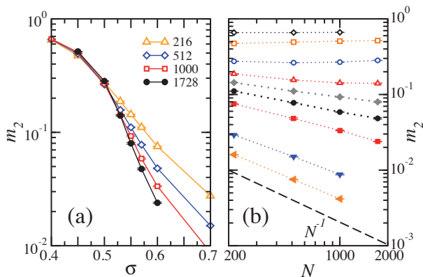
FIG. 12. (Color online) (a) Semilog plots of the squared magnetization m_2 vs \sigma for the lowest available temperature, T = 0.55 . \Delta , \diamond , \square and \circ stand for N = 216, 512, 1000 and 1728 respectively. Solid lines are guides to the eye. (b) Log-log plots of m_2 vs the number of dipoles N at T = 0.55 . From top to bottom, \diamond , \square , \circ , \Delta , \blacklozenge , \bullet , \blacksquare , \blacktriangledown , and \blacktriangleleft stand for \sigma = 0.4, 0.45, 0.5, 0.53, 0.55, 0.57, 0.6, 0.7 , and 0.8 respectively. Dotted lines are guides to the eye. The dashed line shows the N^{-1} decay expected for the paramagnetic phase.
