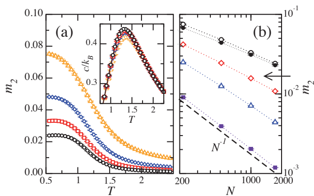
FIG. 7. (Color online) (a) Plots of the squared magnetization m_2 vs T for \sigma = 0.6 . In the inset, the specific heat vs T . \Delta , \diamond , \square and \circ stand for N = 216, 512, 1000 , and 1728 dipoles respectively. All lines in this panel are guides to the eye. (b) Log-log plots of m_2 vs N for \sigma = 0.6 . From top to bottom, \circ , \bullet , \diamond , \Delta , and \blacksquare stand for temperatures T = 0.55, 0.85, 1.25, 1.55 , and 2.55 respectively. The arrow marks the onset of the PM phase. Dotted lines are guides to the eye. The dashed line shows the N^{-1} decay expected for a paramagnet in the thermodynamic limit.
