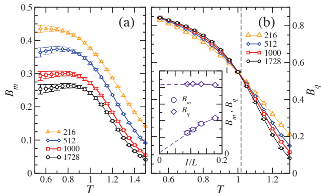
FIG. 9. (Color online) (a) Plots of B_m vs T for \sigma = 0.6 . \Delta , \diamond , \square and \circ mean N = 216, 512, 1000 and 1728 dipoles respectively. The solid lines are guides to the eye. (b) Plots of B_q vs T . Same symbols as in (a). The curves cross at the SG transition temperature, marked in the figure with a vertical dashed line. The inset contains plots of B_m and B_q vs 1/L for the lowest temperature available, T = 0.55 . \circ ( \diamond ) stands for B_m ( B_q ). The dashed lines in the inset are extrapolations.
