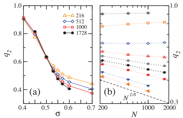
FIG. 13. (Color online) (a) Plots of the squared overlap parameter q_2 vs \sigma for the lowest available temperature, T = 0.55 . \Delta , \diamond , \square and \circ stand for N = 216, 512, 1000 and 1728 respectively. Solid lines are guides to the eye. (b) Log-log plots of q_2 vs the number of dipoles N for T = 0.55 . From top to bottom, \diamond , \square , \circ , \Delta , \blacklozenge , \bullet , \blacksquare , \blacktriangledown , and \blacktriangleleft stand for \sigma = 0.4, 0.45, 0.5, 0.53, 0.55, 0.57, 0.6, 0.7 , and \infty respectively. Dotted lines are guides to the eye. The dashed line corresponds approximately to a N^{-1/8} decay.
