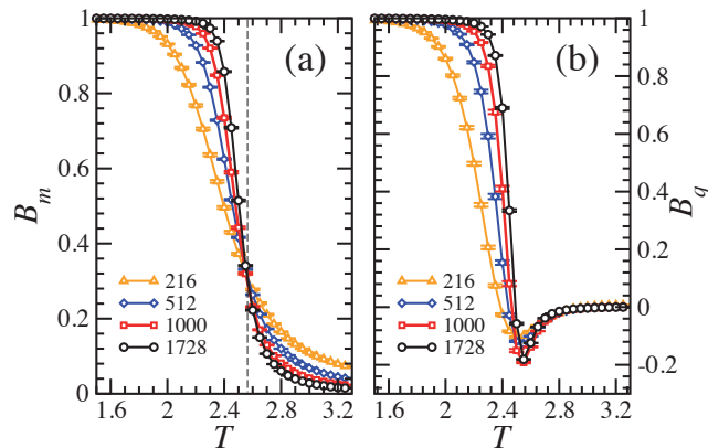
FIG. 5. (Color online) (a) Plots of the Binder cumulant B_m vs T for \sigma = 0.3 . \Delta , \diamond , \square and \circ stand for systems with N = 216, 512, 1000 and 1728 dipoles respectively. The dashed vertical line indicates the Curie temperature, at which curves cross. (b) Plots of the Binder cumulant for the overlap parameter B_q vs T . Same symbols as in (a). Solid lines in both panels are guides to the eye.
