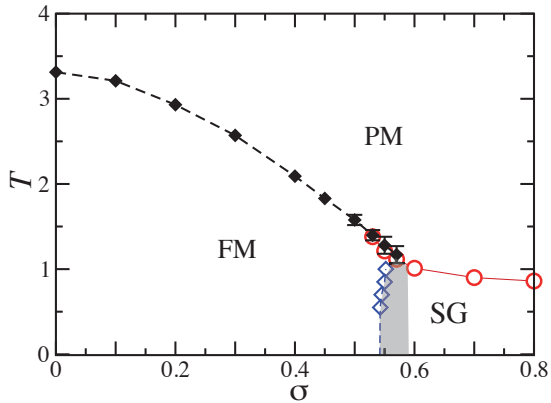
FIG. 2. (Color online) Phase diagram on the temperature-degree of texturation plane for the dipolar Ising model. Symbols \blacklozenge indicate the PM-FM transition and have been obtained from data of B_m vs T . Symbols \circ stand for PM-FM and PM-SG transitions and were obtained from the B_q vs T plots. Symbols \diamond represent the FM-SG transition and follow from the B_m vs \sigma plots. The error bars for the data marked with \circ and \diamond are smaller than the size of these symbols. FM quasi-range order cannot be discarded in the grey region.
