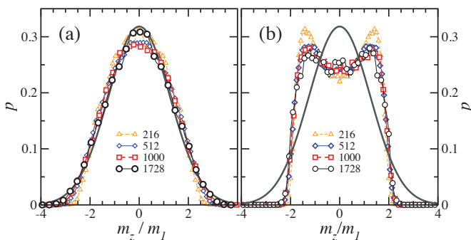
FIG. 10. (Color online) (a) Plots of the probability distribution p(m_z/m_1) for \sigma = 0.6 and T = 0.55 . \Delta , \diamond , \square and \circ stand for N = 216, 512, 1000 and 1728 respectively. The thick solid line is the typical Gaussian distribution for paramagnets in the N \rightarrow \infty limit. (b) Same as in (a) but for \sigma = 0.55 . The thin lines connecting data in both panels are guides to the eye.
