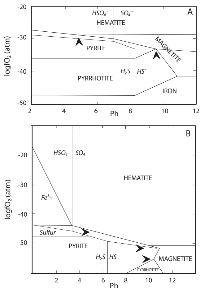
Fig. 14. Log fO_2 versus Ph diagrams for the Fe-S-O system at T = 300 °C (A; Vaughan and Craig 1978), and 125 °C (B; Wang et al. 2010). Arrows delineate the range of redox conditions inferred for NWA 7533.
