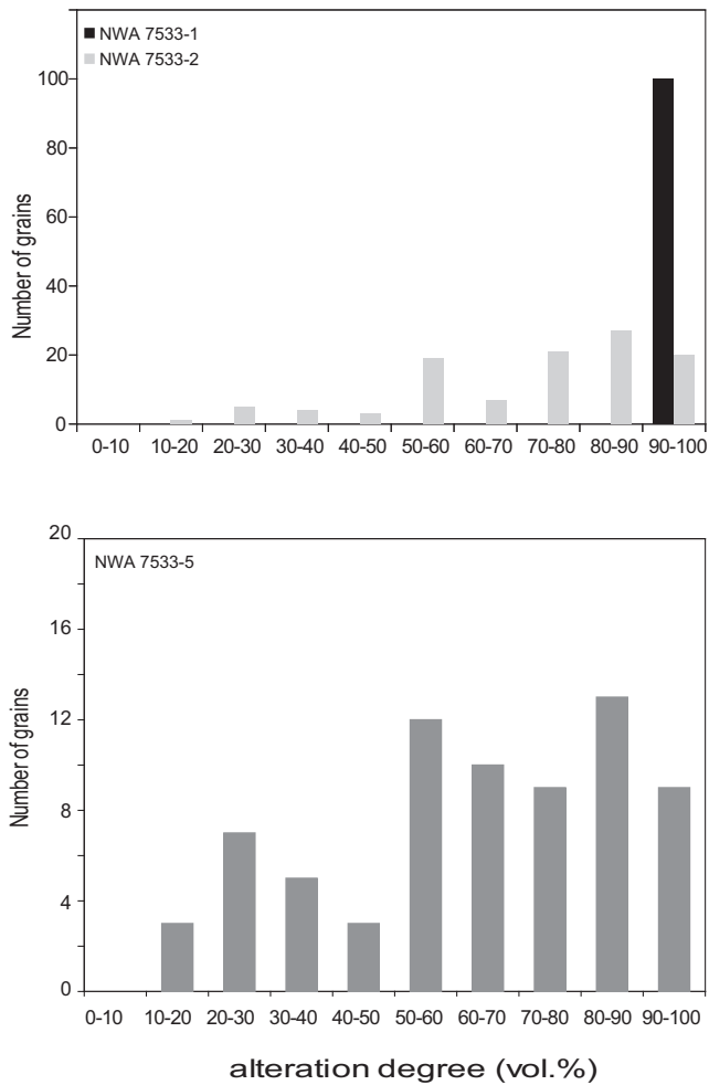
Fig. 6. Histograms showing the alteration degree of pyrite in three polished sections of NWA 7533 (visual estimations from BSE images). Section 1 pyrites are the most altered. Sections 2 and 5 show an alteration gradient from one side to the other, resulting in two pyrite populations with respect to Fe oxyhydroxide alteration.
