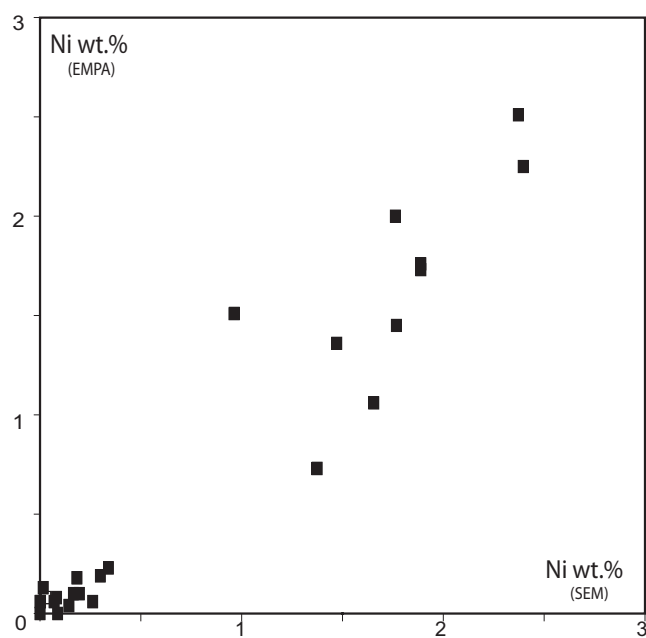
Fig. 10. Comparison between EDS (SEM) and WDS (EMP) analyses of Ni.
